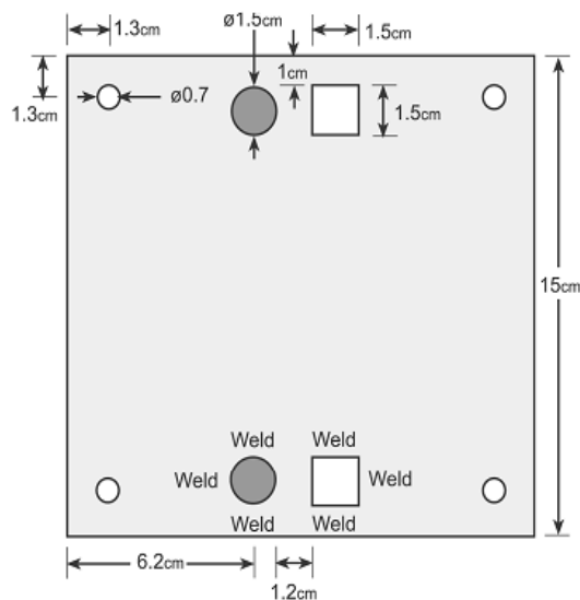
Target Base (plan view)
